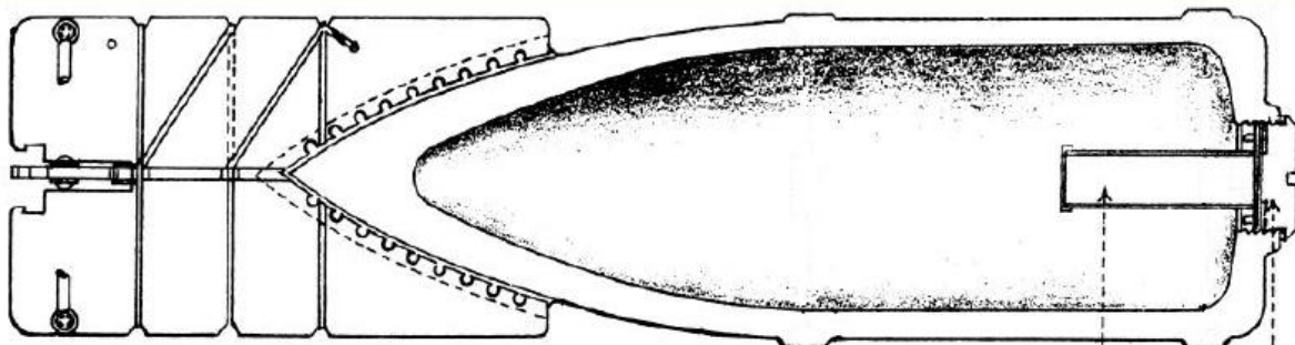
Container exploder H.E. bomb, short Plug Fuze hole 2-inch No 6 A or B
